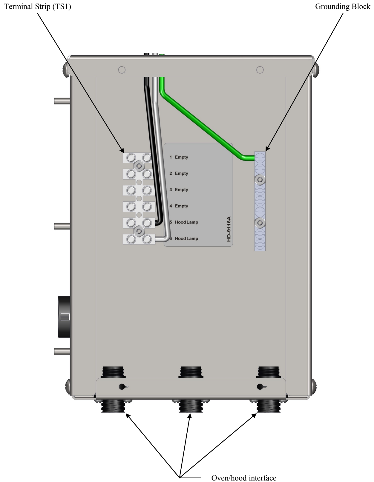
Non-VFD Control Box (Cover removed)
